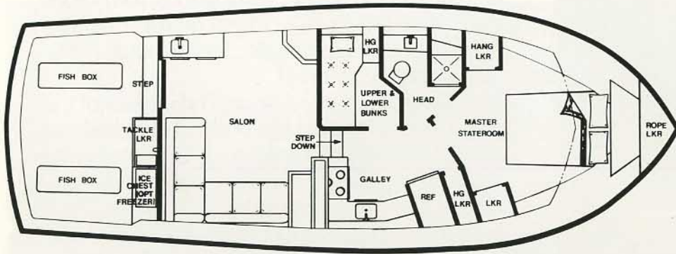
Interior Layout—2 Stateroom Model
