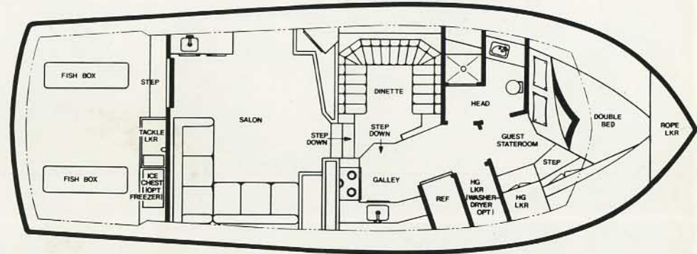
Interior Layout—Dinette Model
